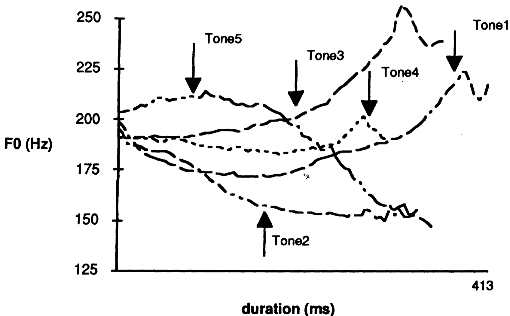
Figure 1. Pitch tracks of five tones in live syllables of KN Lao words in isolation as spoken by a female speaker.
